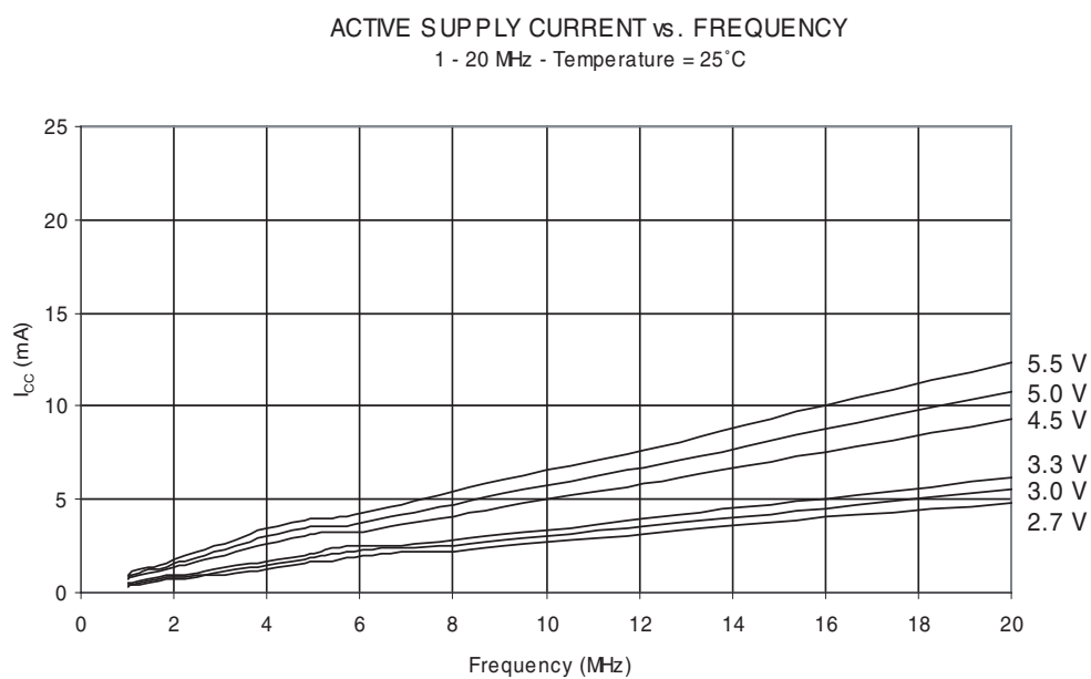
Figure 30-4. Active Supply Current vs. frequency (1 - 20 MHz) - Temp.=125°C
