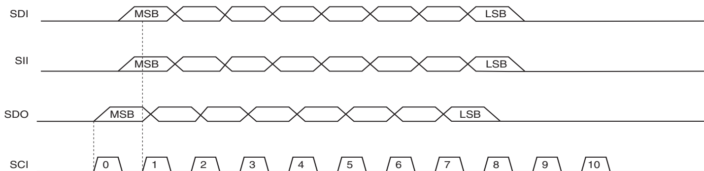
Figure 28-5. High-voltage Serial Programming Waveforms
